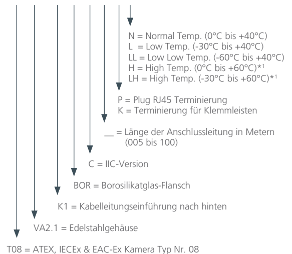
T08-VA2.1.K1.BOR-C-XXX-X-X
