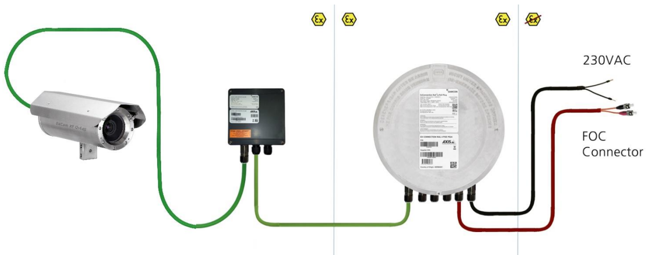
Bild 5-10 ExTB-3 -> ExConnection Rail
