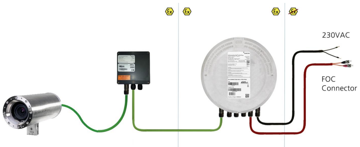
Bild 5-7 ExTB-3 -> ExConnection Rail
