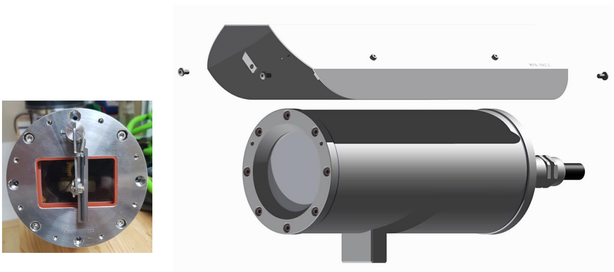
Fig. 6-2 Removing the weather protection roof (2/2) (similar illustration)
